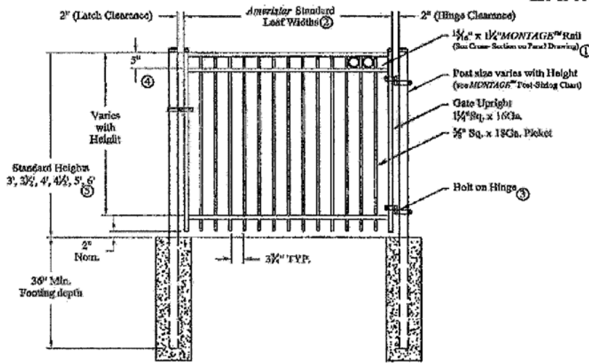
Single gate Arrangement
